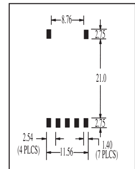
Pad Layout C
