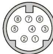
MINIDIN8 – dutinky
