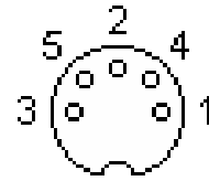
DIN5 – dutinky
