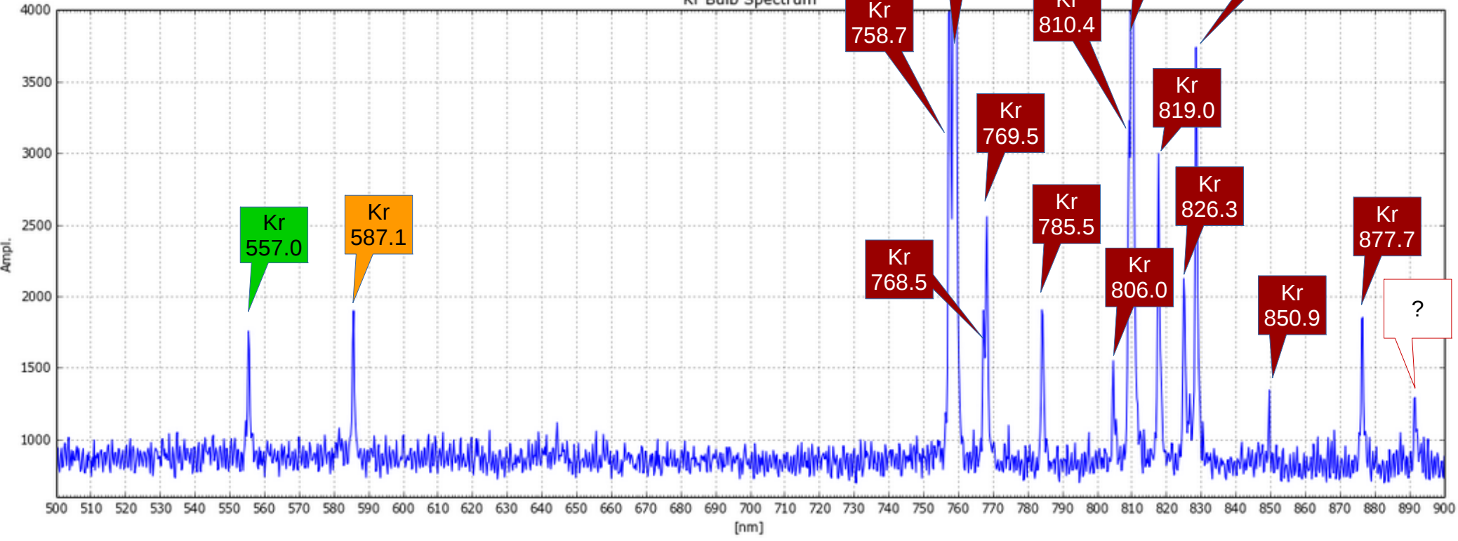
Kr Bulb Spectrum
