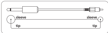
Fig. 5.2: Adapter cable with 1/8" jack
