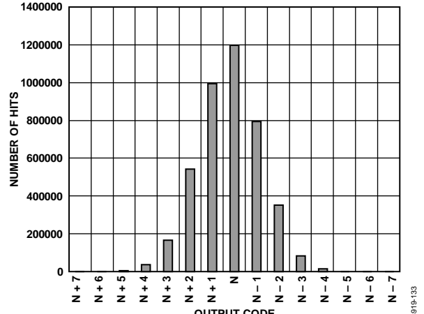
Figure 31. AD9650-65 Grounded Input Histogram
