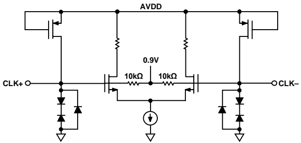
Figure 69. Equivalent Clock Input Circuit
