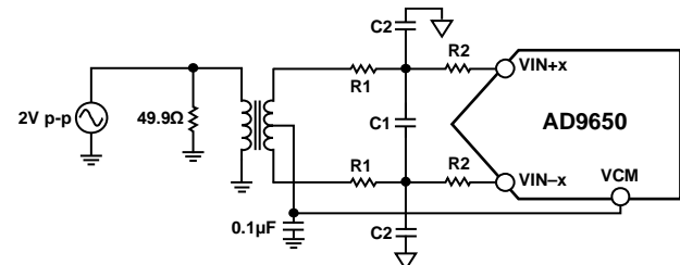
Figure 80. Differential Transformer-Coupled Configuration
