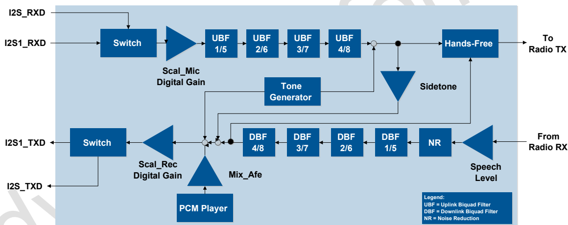
Figure 14: Audio paths
