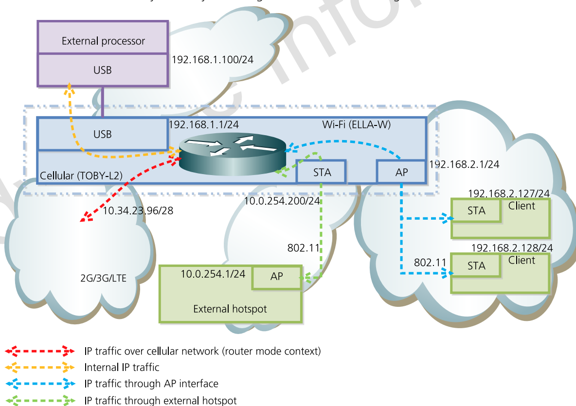
Figure 22: Router mode with Internet access via cellular network or via external hotspot
