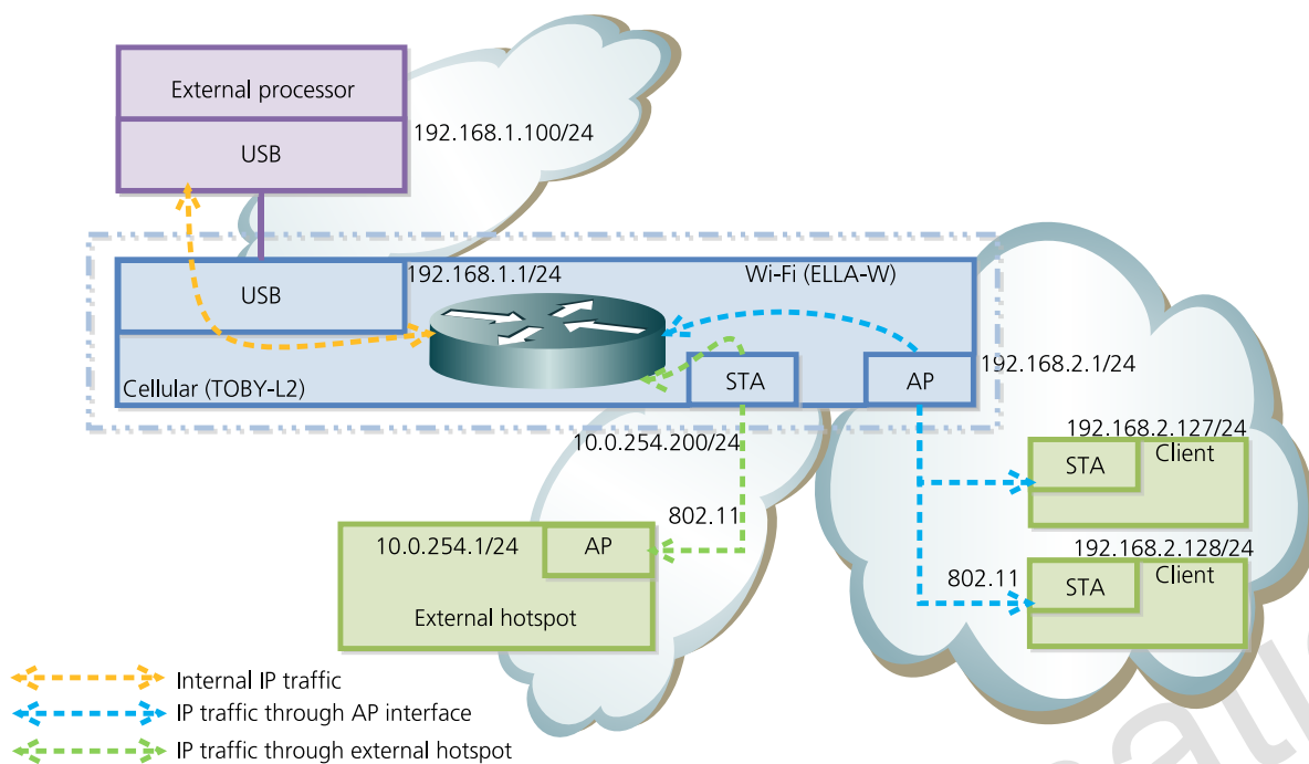
Figure 21: Router mode with Internet access via external hotspot
