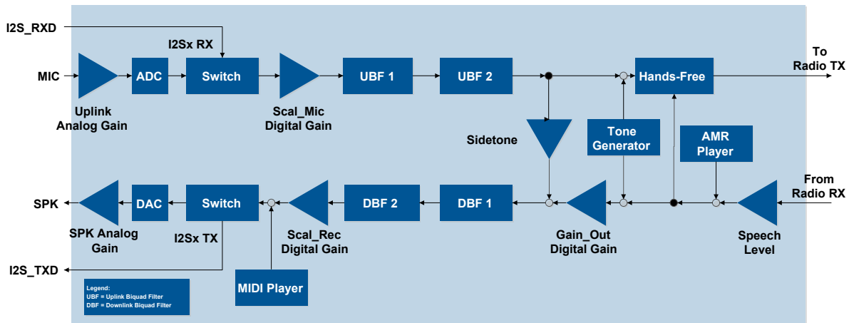
Figure 16: Audio paths
