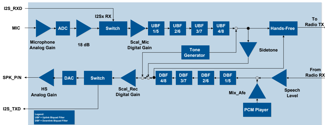
Figure 15: Audio paths
