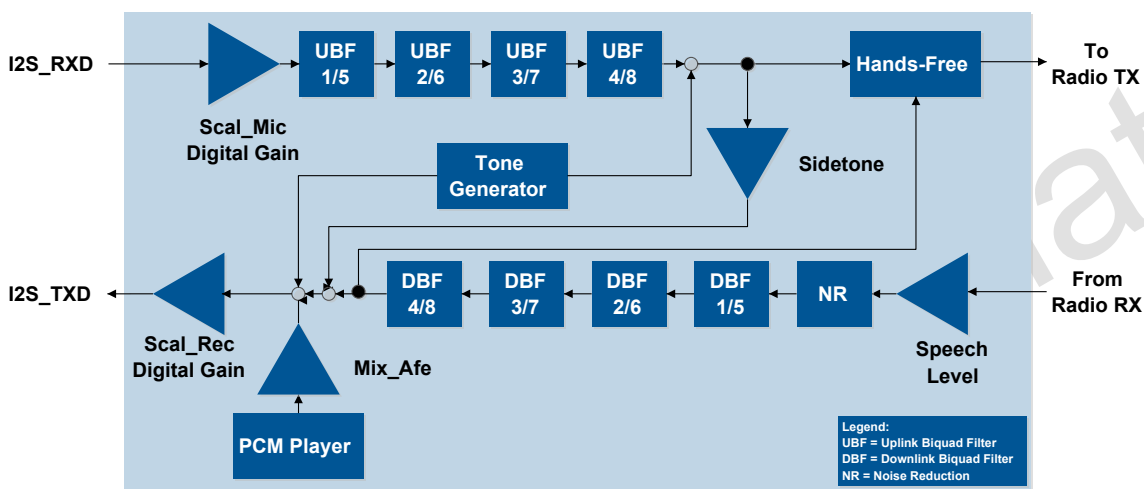
Figure 13: Audio paths
