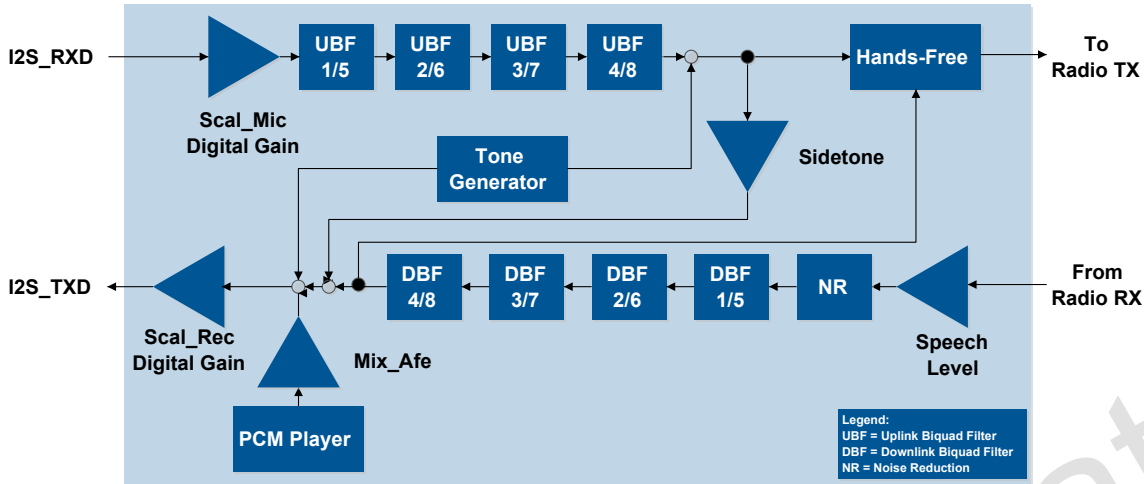
Figure 12: Audio paths
