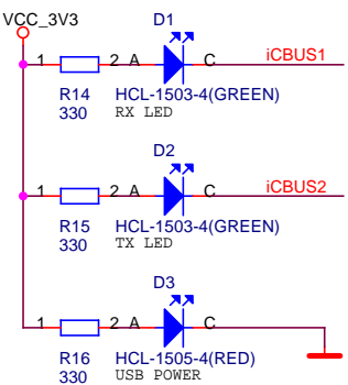
LED INDICATORS
