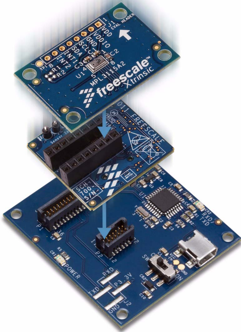
Figure 12. MPL3115A2 daughter board, LFSBEBMPL3115A2 evaluation board and the LSTBUS interface board
