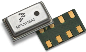
LGA Package 5.0 mm by 3.0 mm by 1.1 mm
