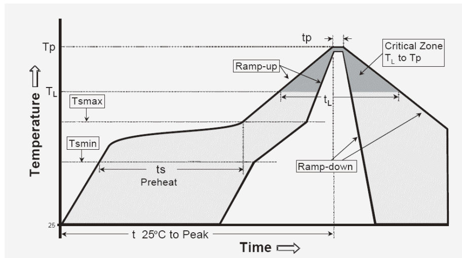
Figure 2: Definitions for reflow profiles
