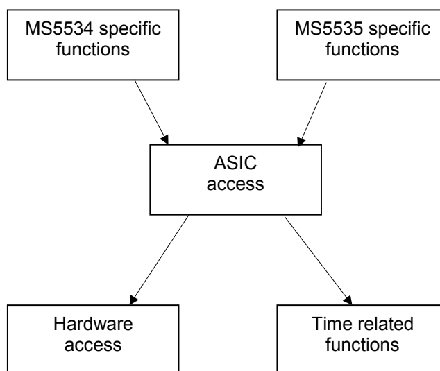
Figure 1. Software hierarchy
