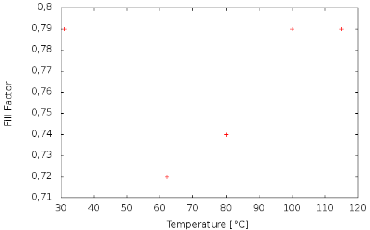
Effect of temperature on a single monocrystal Si cell
