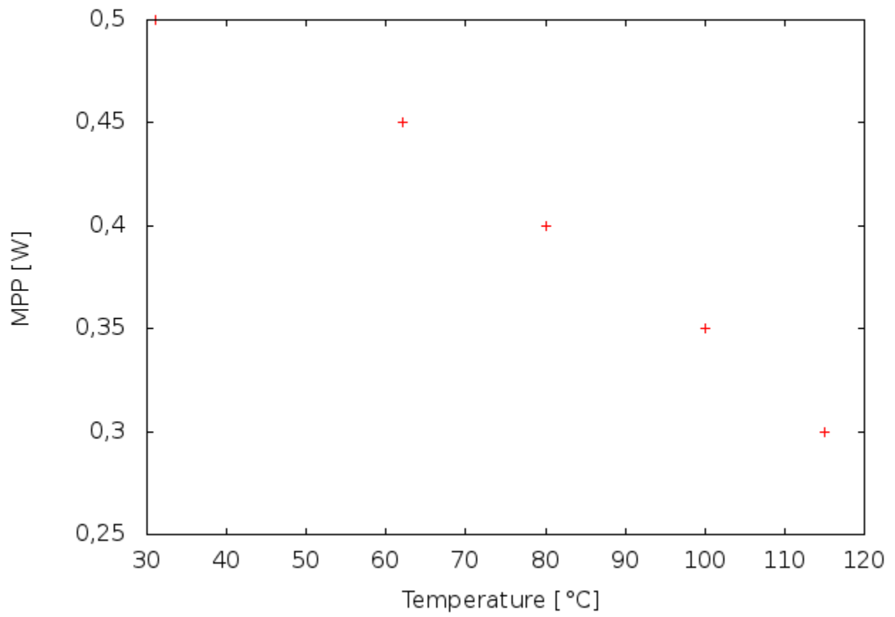
Effect of temperature on a single monocrystal Si cell
