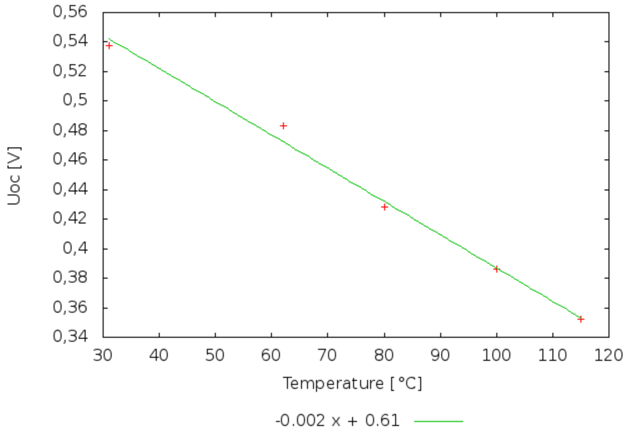
Effect of temperature on a single monocrystal Si cell
