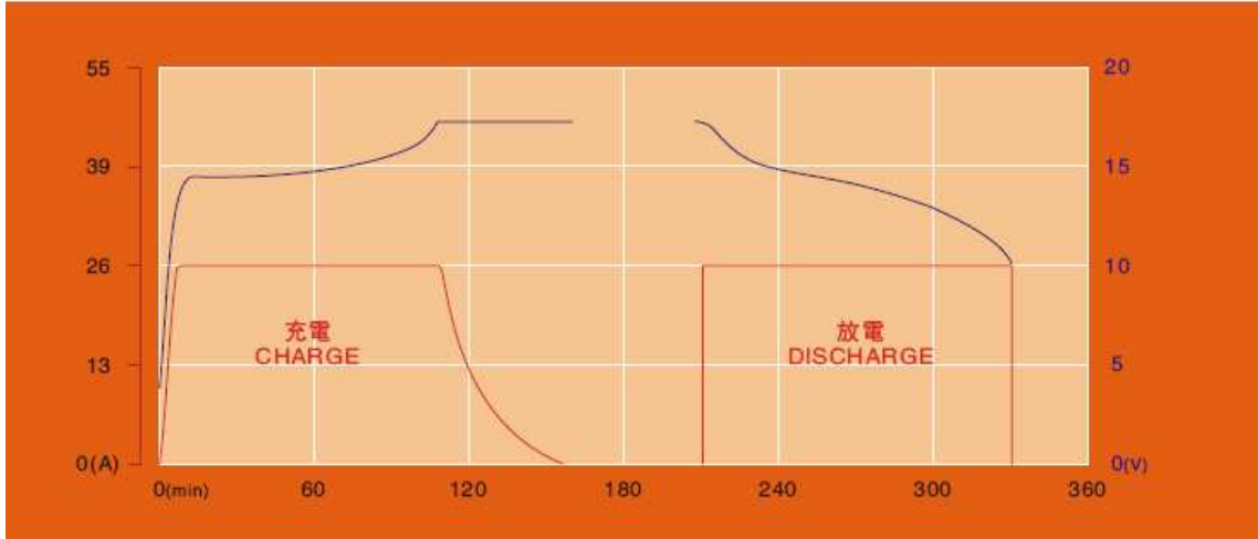
▲ TS-LP12V40AH在25°C環境下26A充放電特性 TS-LP12V40AH CHARGE AND DISCHARGE BY 26A AT TEMPERATURE OF 25°C
