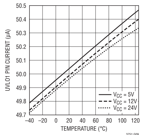
UVL01 Trip Current
