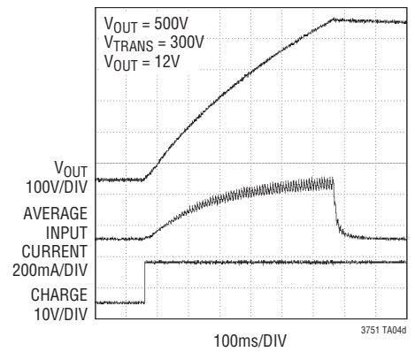
Charging Waveform
