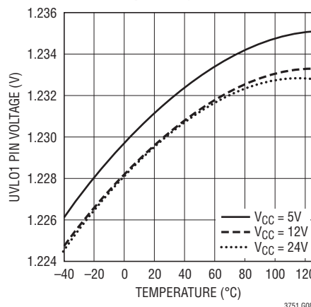
UVL01 Trip Voltage
