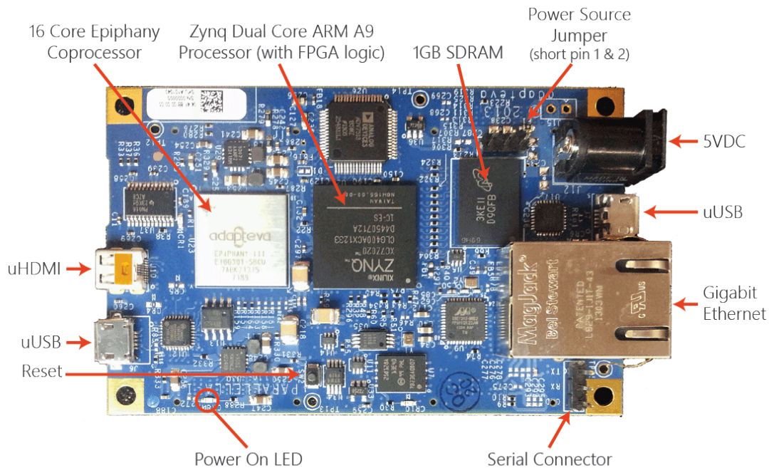
Figure 4.1. Top view on Parallella-16 board [??].
