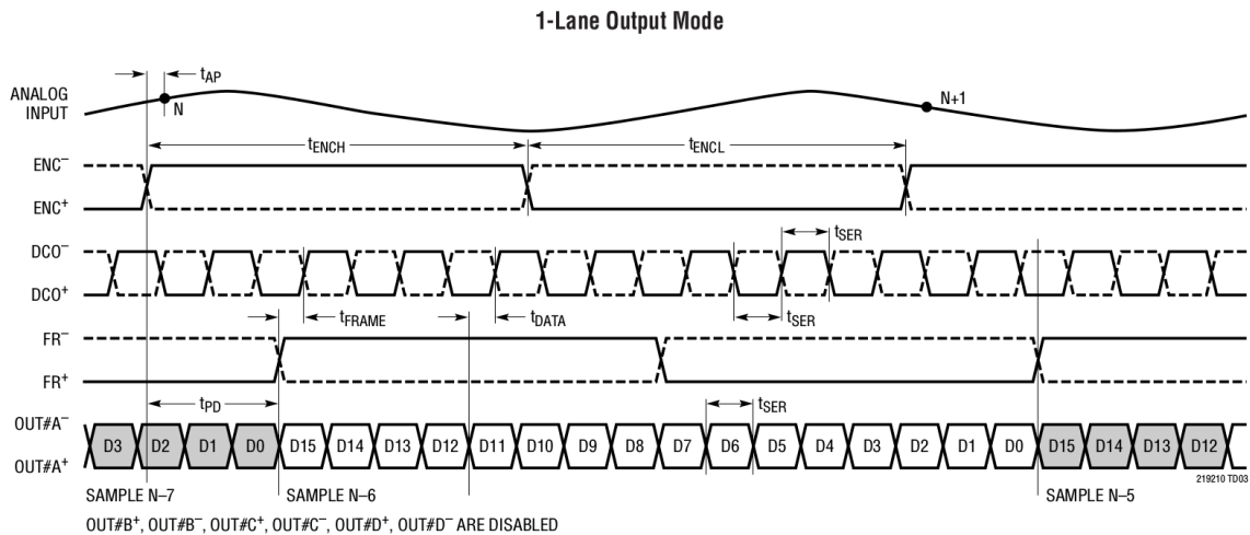
Figure 2.2. Digital signalling schema for 1-line ADC digital output mode.
