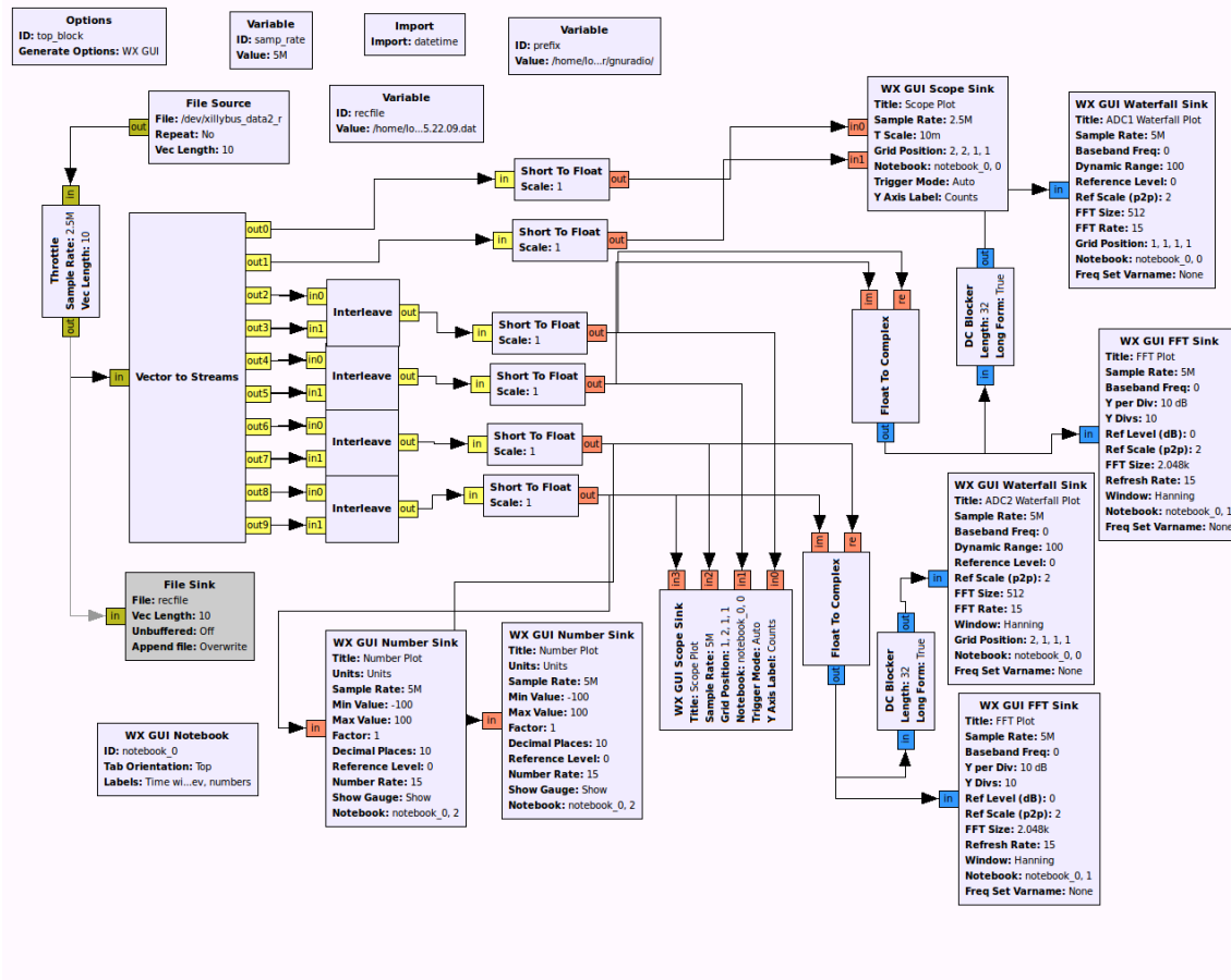
Figure 2.5. An ADC recorder flow graph created in gnuradio-companion.
