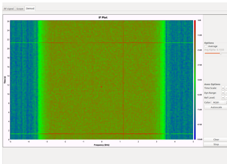
Figure 3.7. Meteor reflection (the red spot in centre of image) received by an evaluation design.
